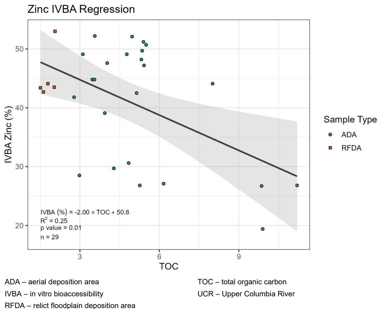
Figure 7. Zinc bioaccessibility as a function of TOC in soils from the UCR Site
